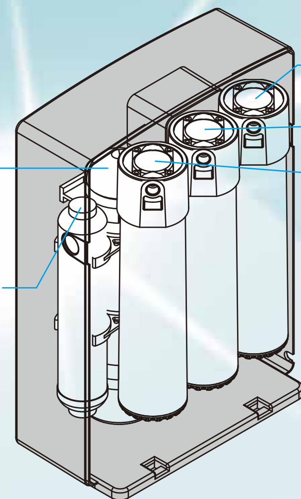
1st PP Filter 2nd GAC Filter 3rd FPC Filter
